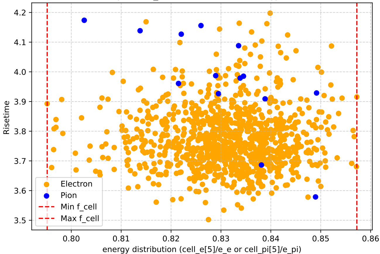
Scatter plot of f_cell vs risetime for energy 40.0GeV
